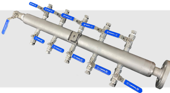
Air distribution manifolds according to PED 2014/68/EU
