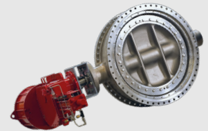
Butterfly Valve Triexcentric
