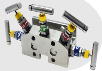
2 Way 5 Valves
